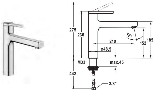
Art.-No. KWC-No. FUN 125361 10.461.022.000FL all chrome, A 210, flexible connection hoses
