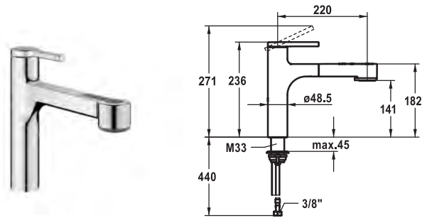
Art.-No. KWC-No. FUN 125364 10.461.032.000FL all chrome, A 220, flexible connection hoses
